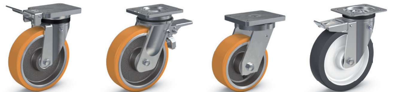
PEVOPUR® industrial guiding castors Series 223 PEVOPUR® heavy-duty guiding castors Series 191 PEVOPUR® heavy-duty guiding castors Series 195 PEVOTHAN® industrial guiding castors with spring-loaded directional locks Series 51 PU/NI
