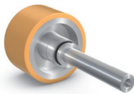
VULKOLLAN® drive wheels with axle Series 178 A/173 A
